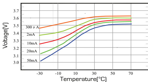
Voltage vs Temperature
